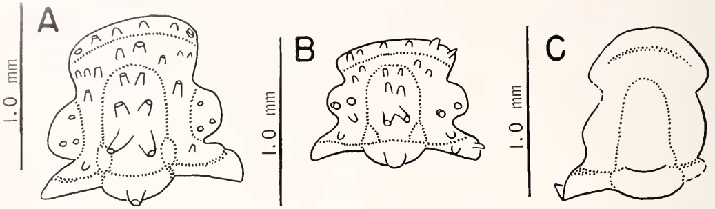
Figure 6. Smallest cranidia in size series showing some paired spines. A) Otarion instita n. sp. (original of Pl. 6, figs. 18, 19, 24). B) Otarion plautum n. sp. (original of Pl. 7, figs. 19, 24, 25). C) Proetus pluteus n. sp., USNM 154491, slightly smaller than original of Plate 1, figs. 23, 24, 30, 31.
